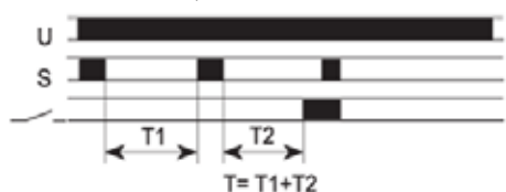
FZ09: ON delay, additive
