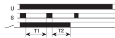
FZ10: Signal ON pulse+OFF pulse, additive
