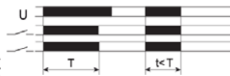
FZ19: ON pulse (1 timed contact + 1 instantaneous contact)
