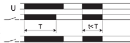
FZ20: Fixed pulse (0.5s) delayed
