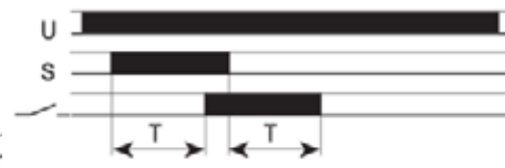
FZ16: ON Delay (1 timed contact + 1 instantaneous contact)
