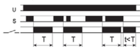
FZ07: Signal OFF pulse
