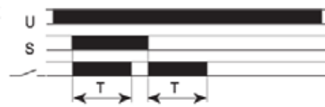
FZ12: Signal ON and OFF delay
