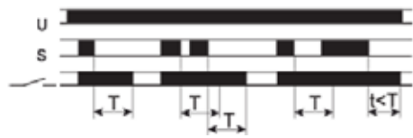
FZ03: Symmetrical recycling: ON start
