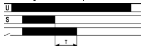
FZ73: Pulse forming fuction
