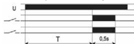
FZ20: Fixed pulse (0.5s) delayed
