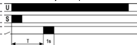
FZ79: Symmetrical recycling with instantaneous contact
